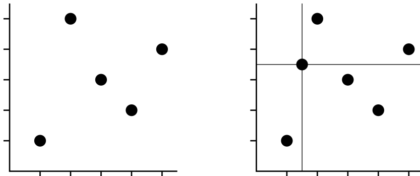
Figure 2: ins(15324, 2, 4) = 146325 .
