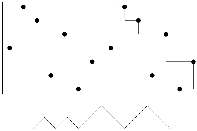
Figure 1: \phi(4762513) = UDUDUDDUDD
