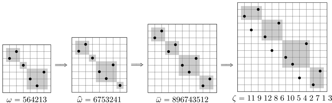
Figure 3: The progression from \omega to \zeta , when \pi has a corner point, as described in the proof of Lemma 2.1.
