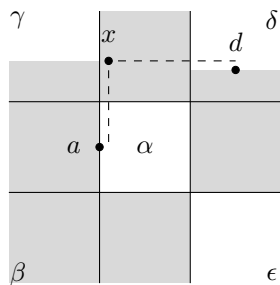
Figure 27: A diagram of the second case in the proof of Theorem 3.9
