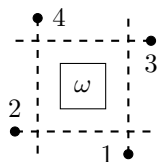
Figure 4: The embedding of \omega into \zeta in the case where \omega does not have a corner point as described in the proof of Lemma 2.1.
