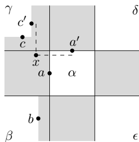
Figure 9: The diagram for Case 2a in the proof of Theorem 3.3.
