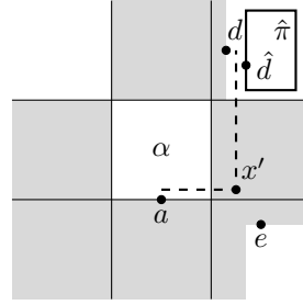
Figure 24: A diagram corresponding to \omega^+ in the second case of Theorem 3.7.
