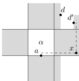
Figure 29: The permutation diagram of \omega^+ in Proposition 3.10.
