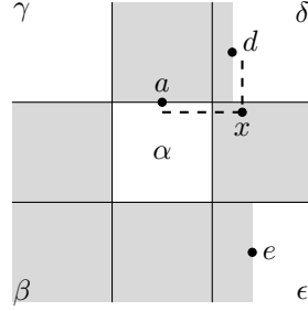
Figure 19: A diagram corresponding to \omega^+ in the first case of Theorem 3.6.
