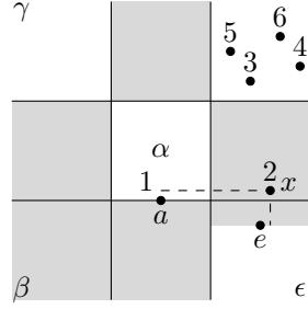
Figure 17: A diagram showing a possible occurrence of \pi in Theorem 3.5.
