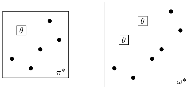
Figure 30: The permutations \pi^* (on the left) and \omega^* (on the right).
