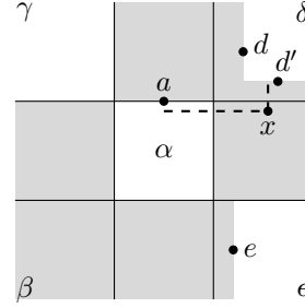
Figure 20: A diagram corresponding to \omega^+ in the second case of Theorem 3.6.
