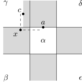
Figure 7: The permutation \omega^+ formed by inserting the entry x into \omega just to the left of c and just below a , in the proof of Theorem 3.2
