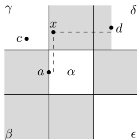
Figure 15: The diagram corresponding to the second part of Case 2 in the proof of Theorem 3.4.
