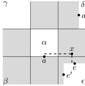
Figure 21: A diagram corresponding to \omega^+ in the first case of Theorem 3.7.
