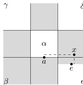
Figure 16: The diagram corresponding to an initial placement of x in Theorem 3.5.
