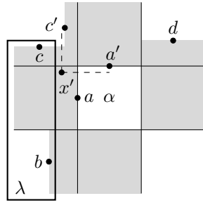
Figure 11: A diagram showing the existence of an occurrence of \lambda in \omega as in Case 2b of Theorem 3.3.
