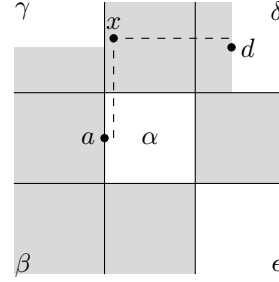
Figure 14: The diagram corresponding to the first part of Case 2 in the proof of Theorem 3.4.
