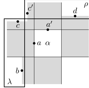
Figure 12: A diagram showing the existence of an occurrence of \pi in \omega as in Case 2b of Theorem 3.3.
