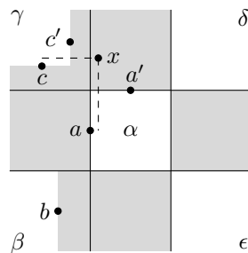
Figure 10: The first diagram for Case 2b in the proof of Theorem 3.3.
