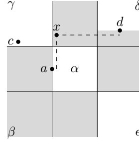
Figure 26: A diagram of the first case in the proof of Theorem 3.9
