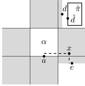
Figure 23: A diagram corresponding to \omega^+ in the second case of Theorem 3.7.
