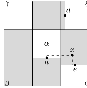
Figure 22: A diagram corresponding to \omega^+ in the second case of Theorem 3.7.
