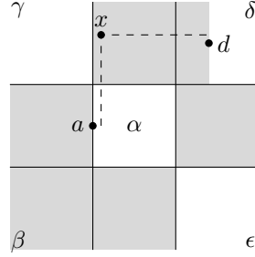
Figure 13: The diagram corresponding to Case 1 in the proof of Theorem 3.4.
