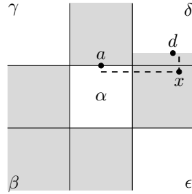
Figure 25: A diagram corresponding to \omega^+ in Theorem 3.8.
