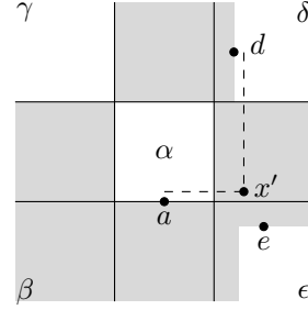
Figure 18: The new placement of a splitting entry in the proof of Theorem 3.5.
