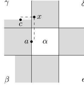
Figure 8: The diagram for Case 1 in the proof of Theorem 3.3.
